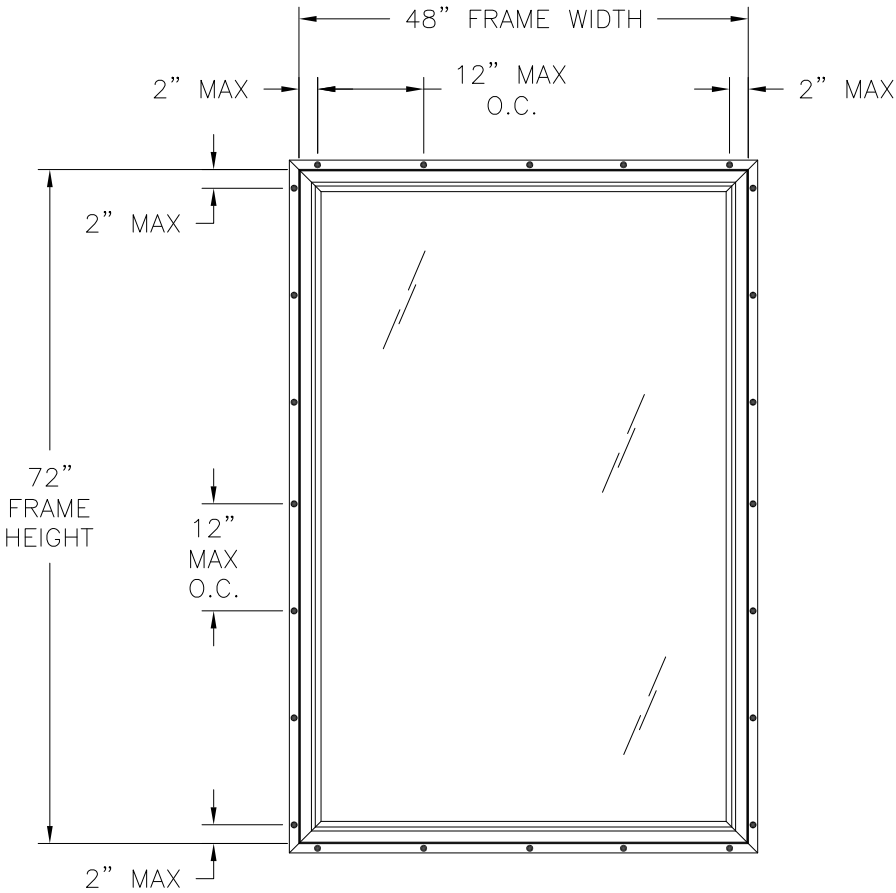
200/275 VINYL PICTURE WINDOW EXTERIOR VIEW
